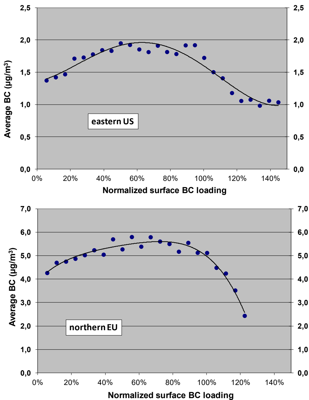
Figure 3: Loading effect in another filter-based BC-measuring instrument. Data sorted and averaged according to cumulative loading on spot; 1 month of data from the eastern US (top), and 1 week of data from northern Europe (bottom).
