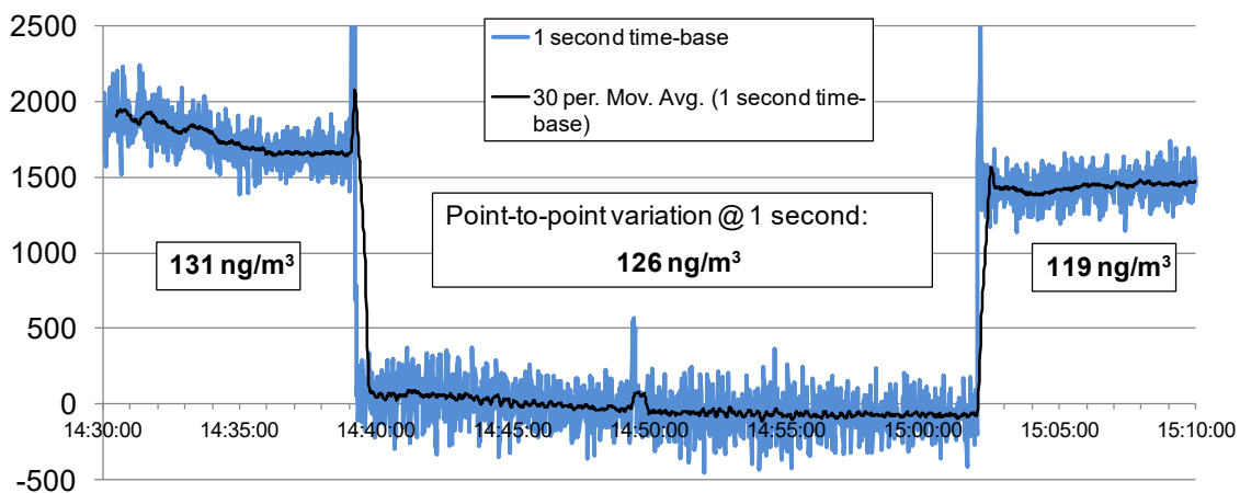
Figure 4: 'Zero-air' check. The Model AE33 Aethalometer switches from sampling ambient air to filtered air. One-second data is 60 times noisier than the one-minute average.
