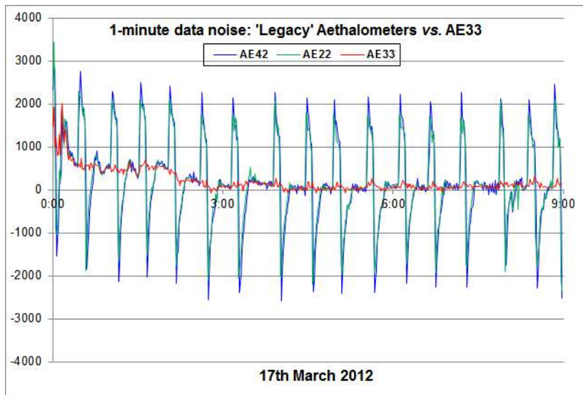
Figure 6: Perturbation of data induced by fluctuation in room air Relative Humidity when subject to an on-off cycling air-conditioner. “Legacy” instruments using quartz fiber tape show large perturbation, while the effects on the AE33 are greatly reduced. However, a Sample Stream Dryer (optional accessory) is recommended for best results.
