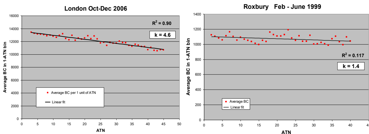
Figure 1: Aethalometer data sorted and averaged according to loading (attenuation, ATN) on spot. Left: roadside location in London, UK; right: urban site in Boston (Roxbury), USA.
