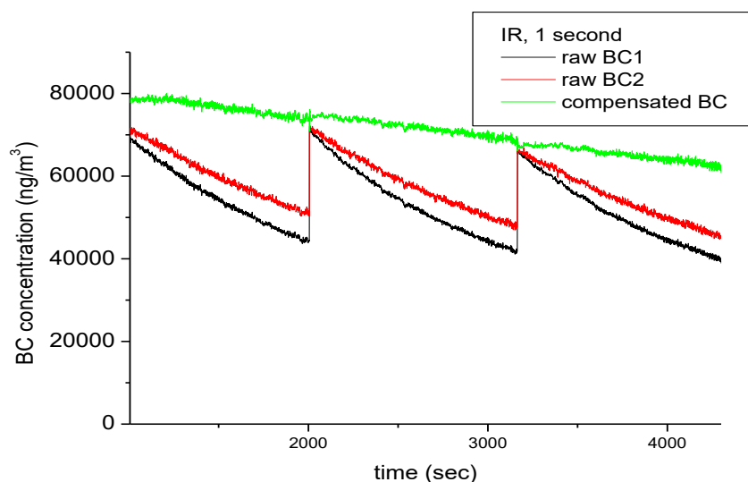
Figure 2: The time-series of AE33 raw and compensated BC concentrations with 1 second timebase – note the extreme concentrations and loading effects.
