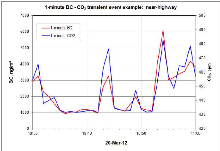
Figure 9: Highly-correlated BC and CO 2 data from integrated sensor with combined data stream. The correlations permit a determination of the BC Emission Factor of the source creating the transient plume.
